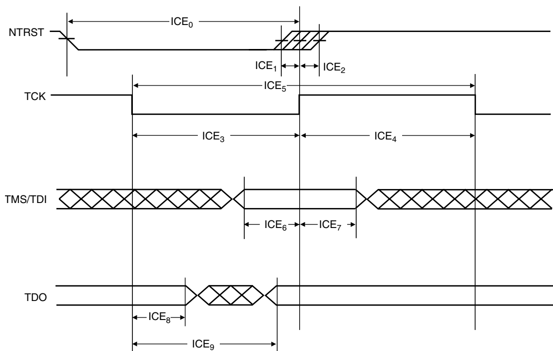
Figure 11. ICE Interface Signals
