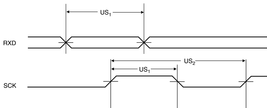
Figure 6. USART Signals
