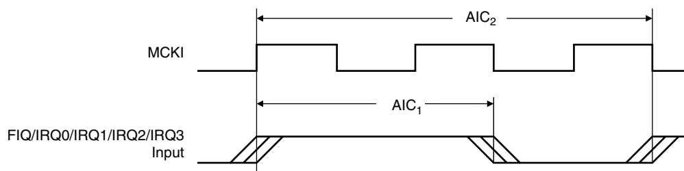
Figure 9. AIC Signals
