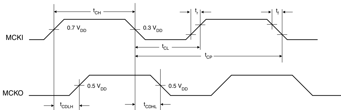
Figure 3. Clock Waveform
