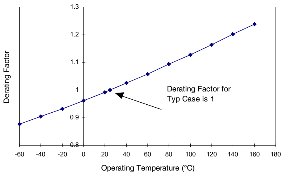
Figure 1. Derating Curve for Different Operating Temperatures
