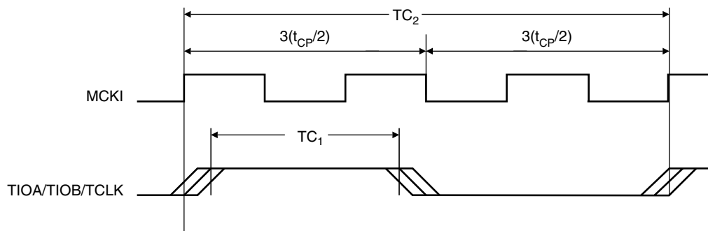
Figure 7. Timer Input
